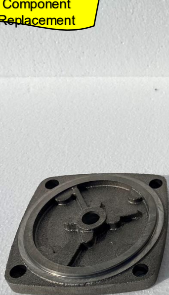
Water Mixing Valve Body and Cover Gray Cast Iron Components, 13.9 kg
