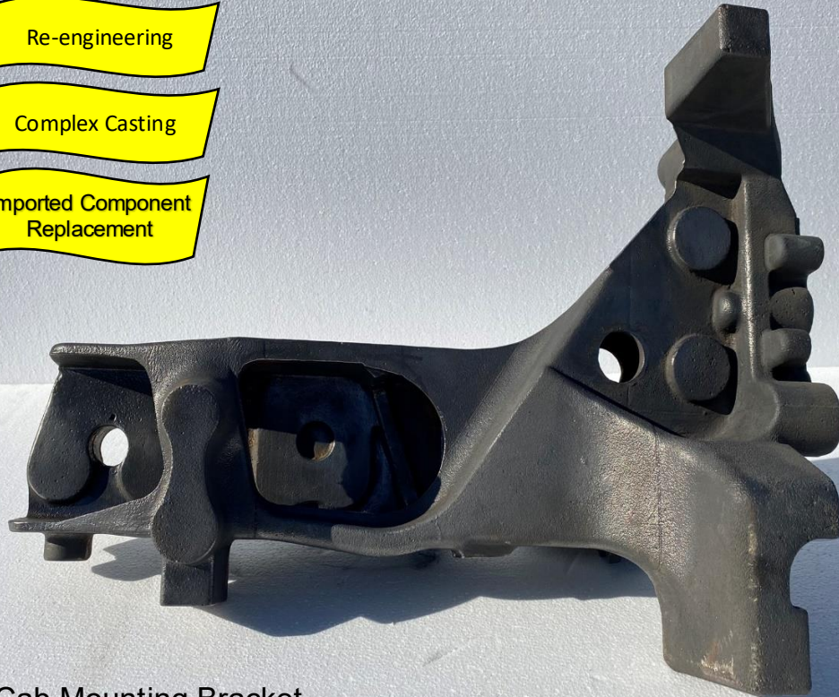
Cab Mounting Bracket Hollow Ductile Iron Casting, 26.2 kg
