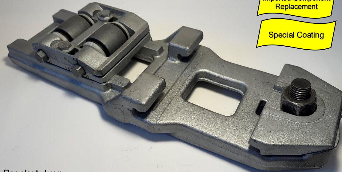
Bracket, Lug, Roller Stop Ductile Iron Components, 12.5 kg
